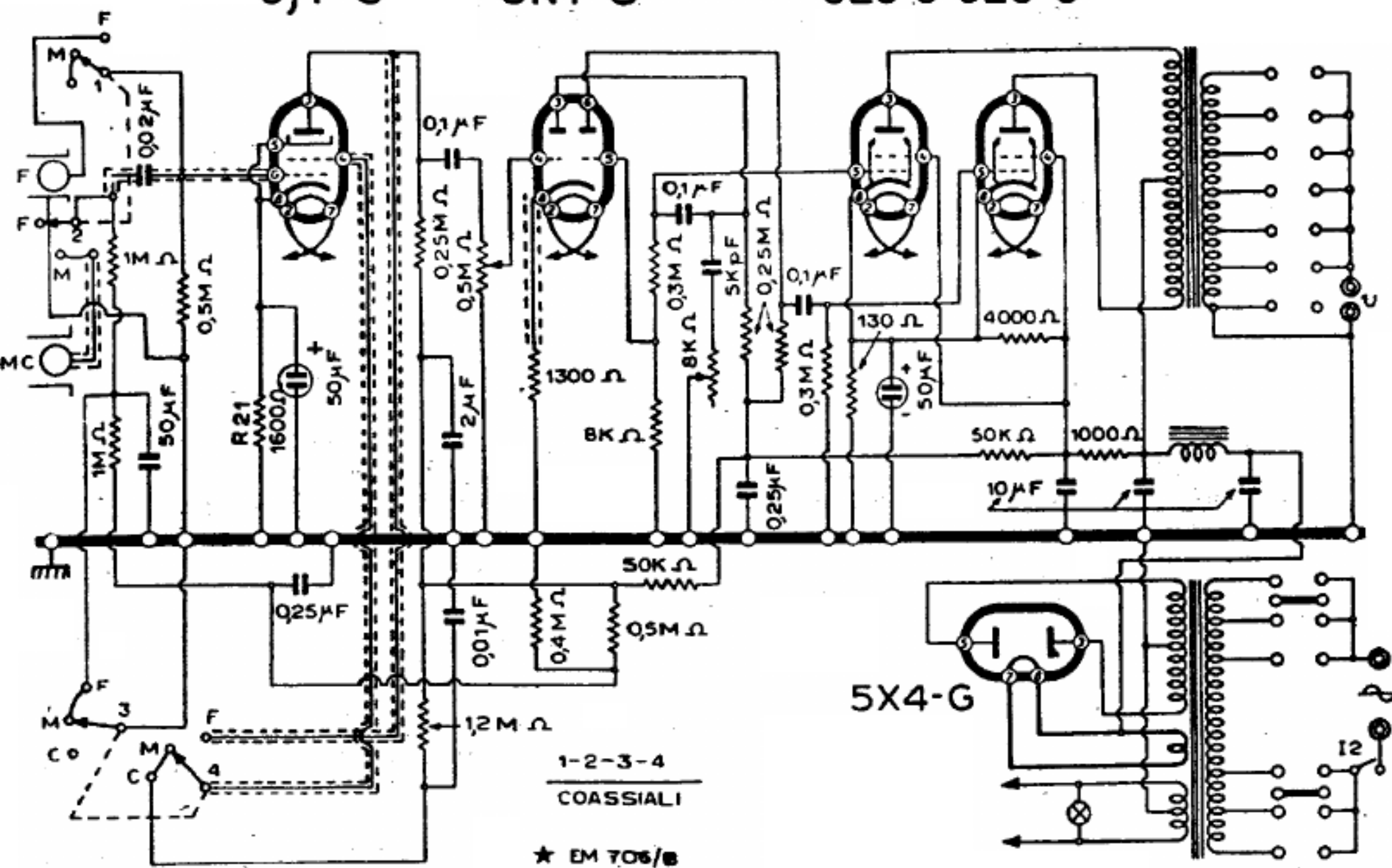
Ducati RG2501-2 Amplifier
